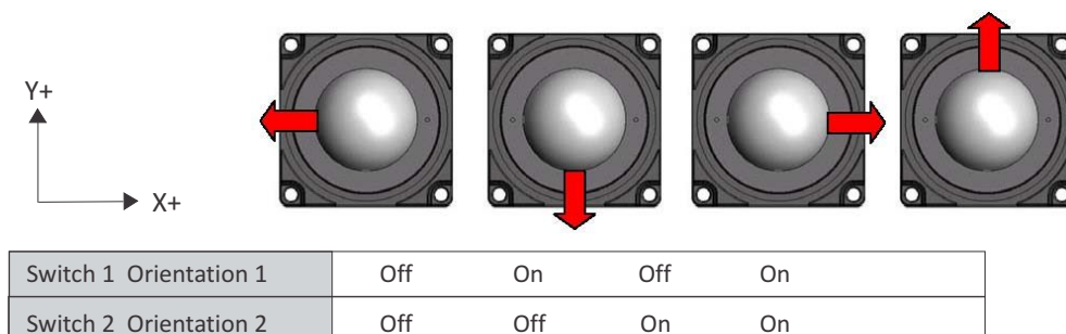
Figure.1 Mounting Orientations
