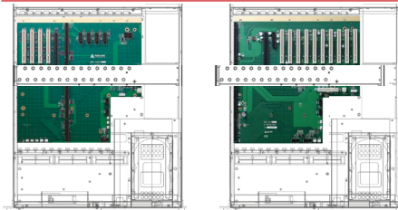
EBP-10E5 1 x PICMG CPU, 1 x PCI-E x16, 4 x PCI-E x1, 4 x PCI
