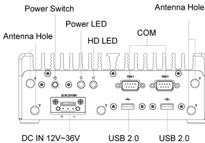
Rear Panel
