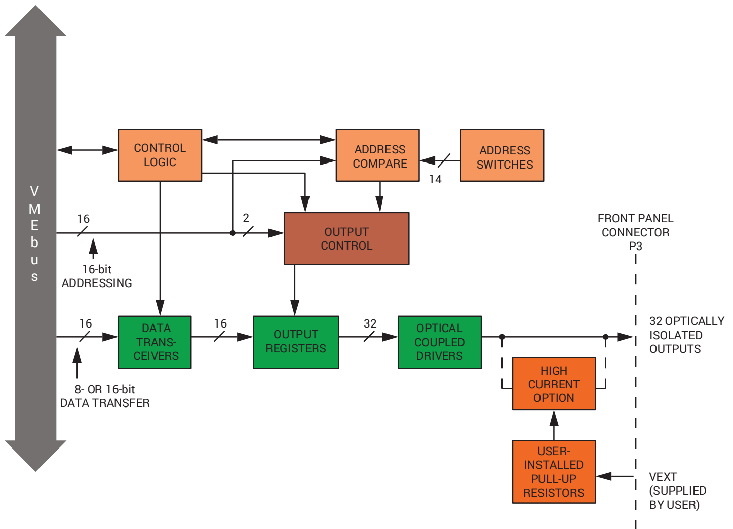
Figure 2. VMIVME-2170A Functional Block Diagram
