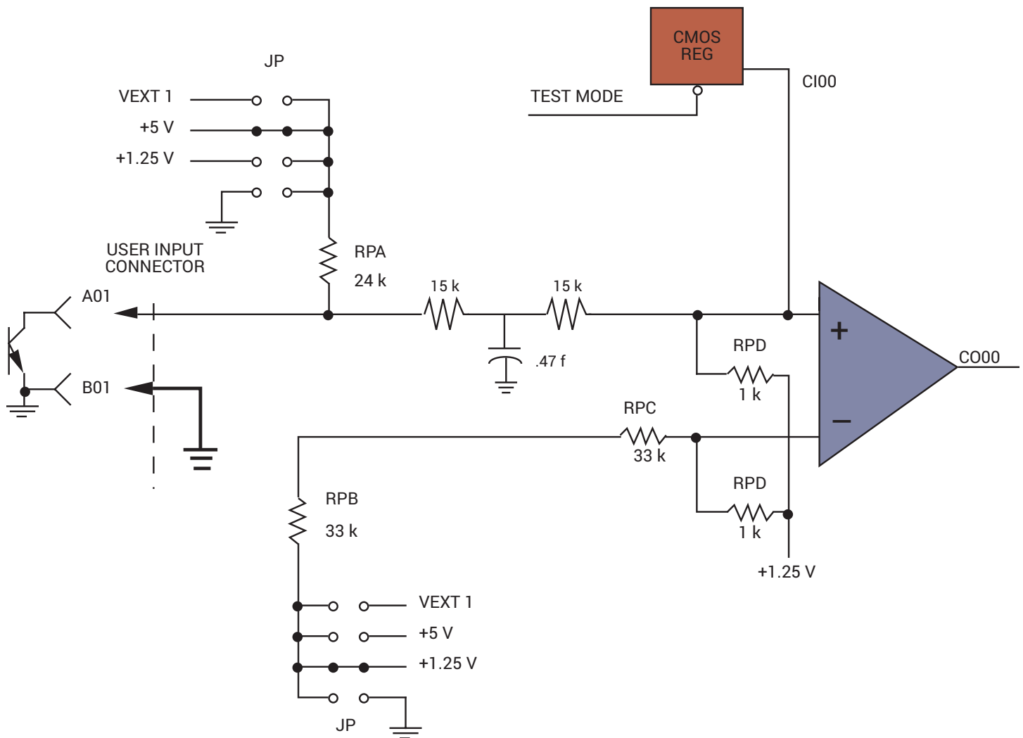
Figure 5. Input Configuration for Current Sinking Inputs
