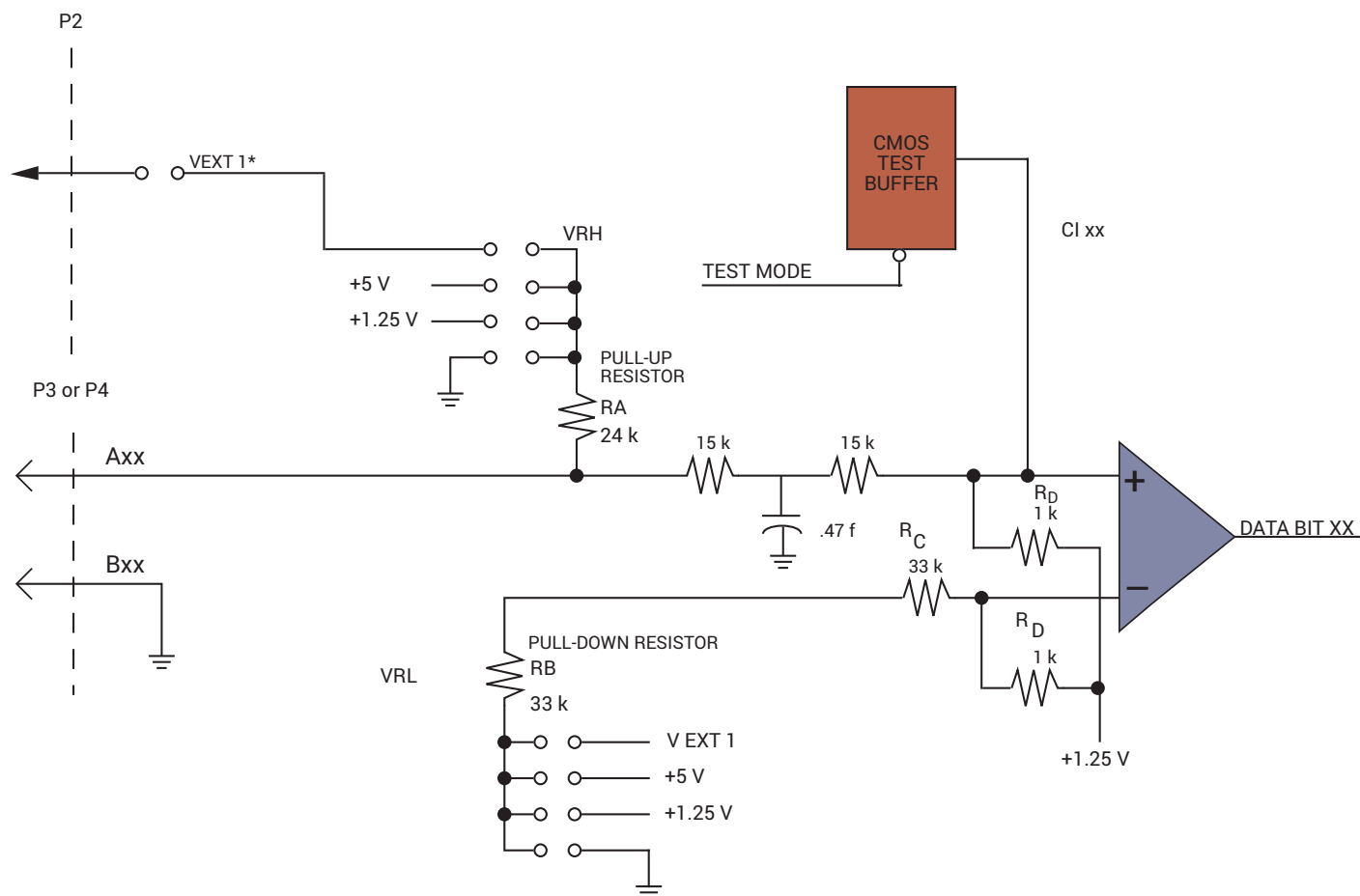
Figure 2. Typical Input Signal Conditioning
