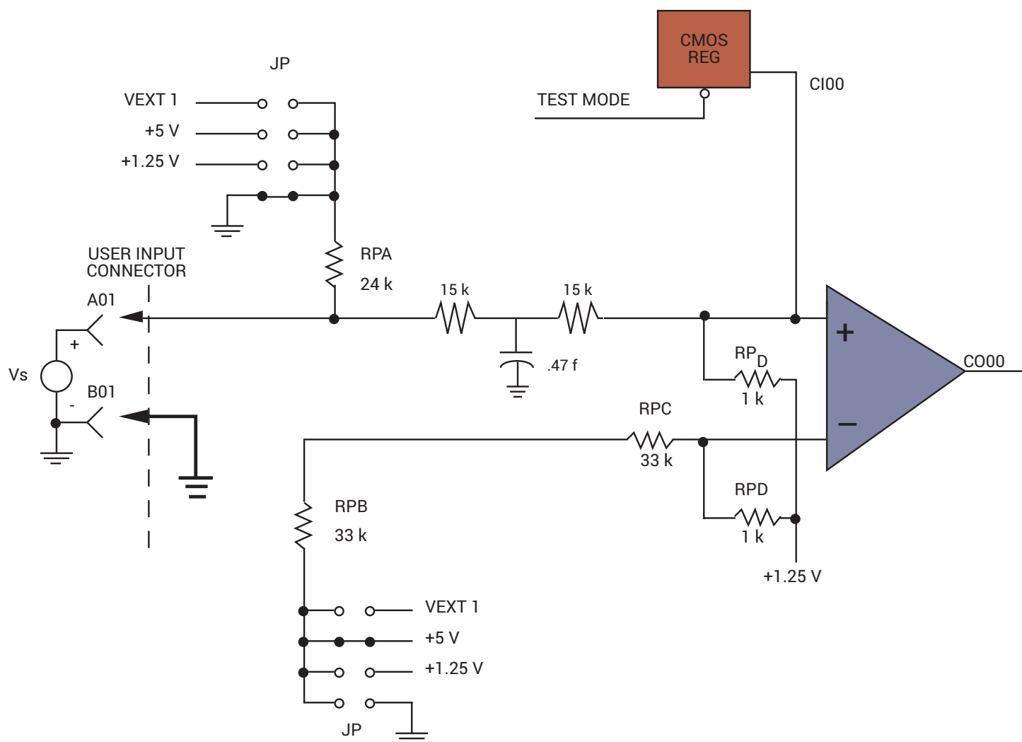
Figure 4. Input Configuration for Voltage Sourcing Inputs
