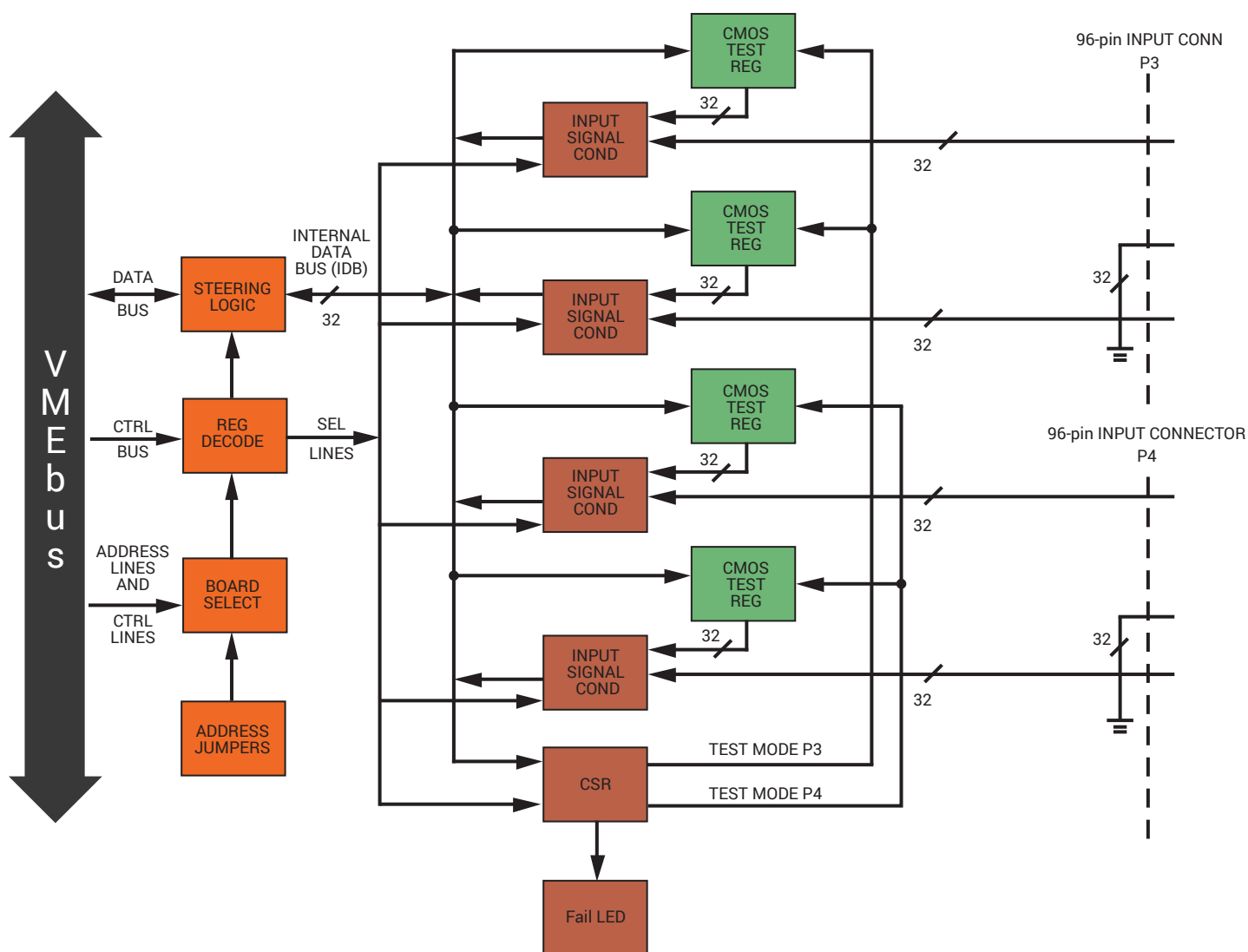
Figure 1. Block Diagram of the VME-1129
