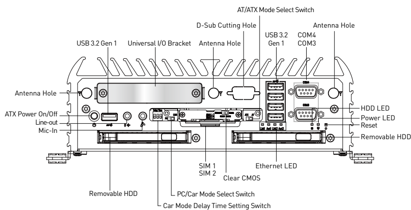
Front Panel
