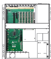
EBP-9E2 1 x PICMG CPU 1 x PCI-E x16, 1 x PCI-E x4, 6 x PCI
