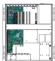
EBP-5E1 1 x PICMG CPU, 1 x PCI-E x16, 1 x PCI-X, 2 x PCI
