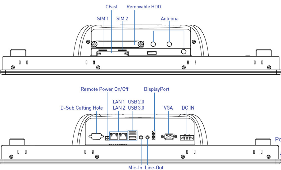
Rear I/O
