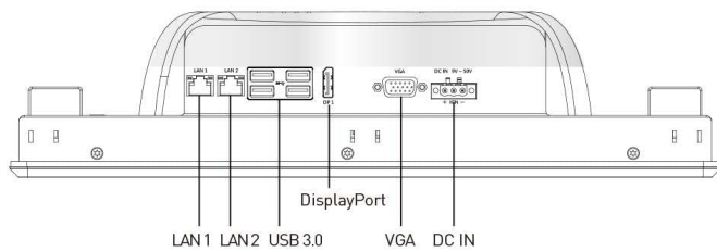
Rear I/O
