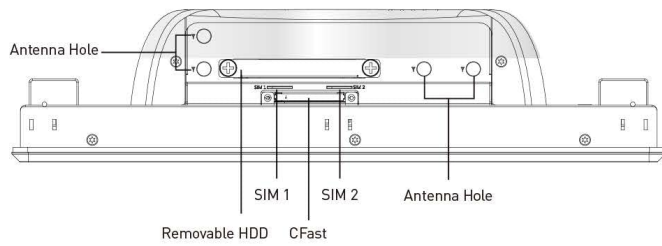
Front I/O
