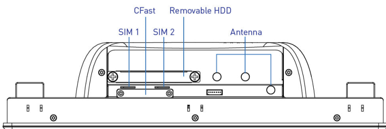
Rear I/O
