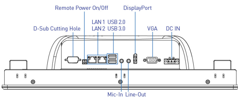
Rear I/O
