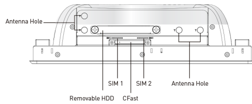
Front I/O
