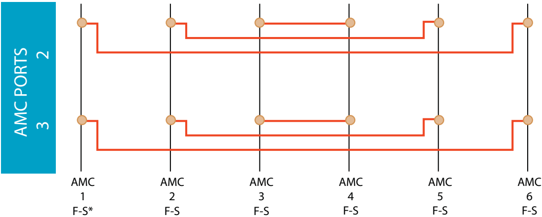
Topology for Ports 2 and 3 with direct connections among the slots (ordering option)
