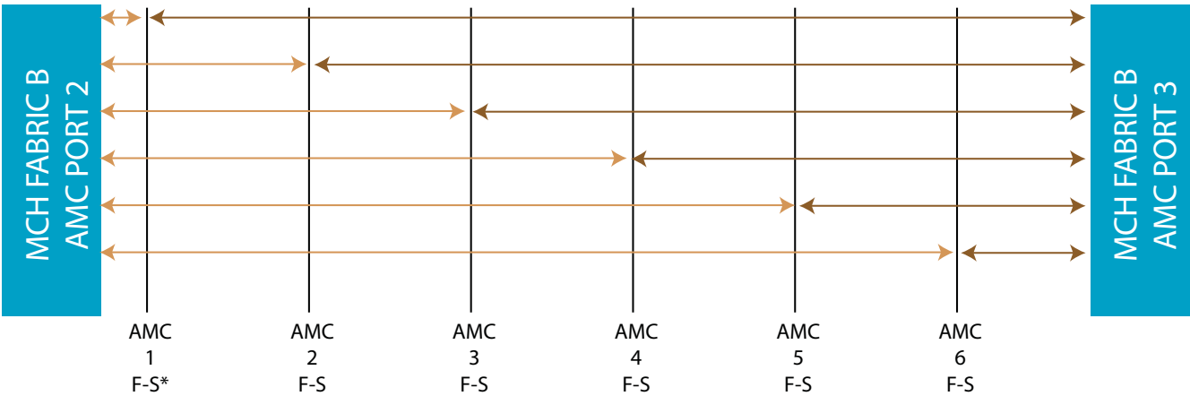
Topology for Ports 2 and 3 to MCH (ordering option for direct connection between the ports)
