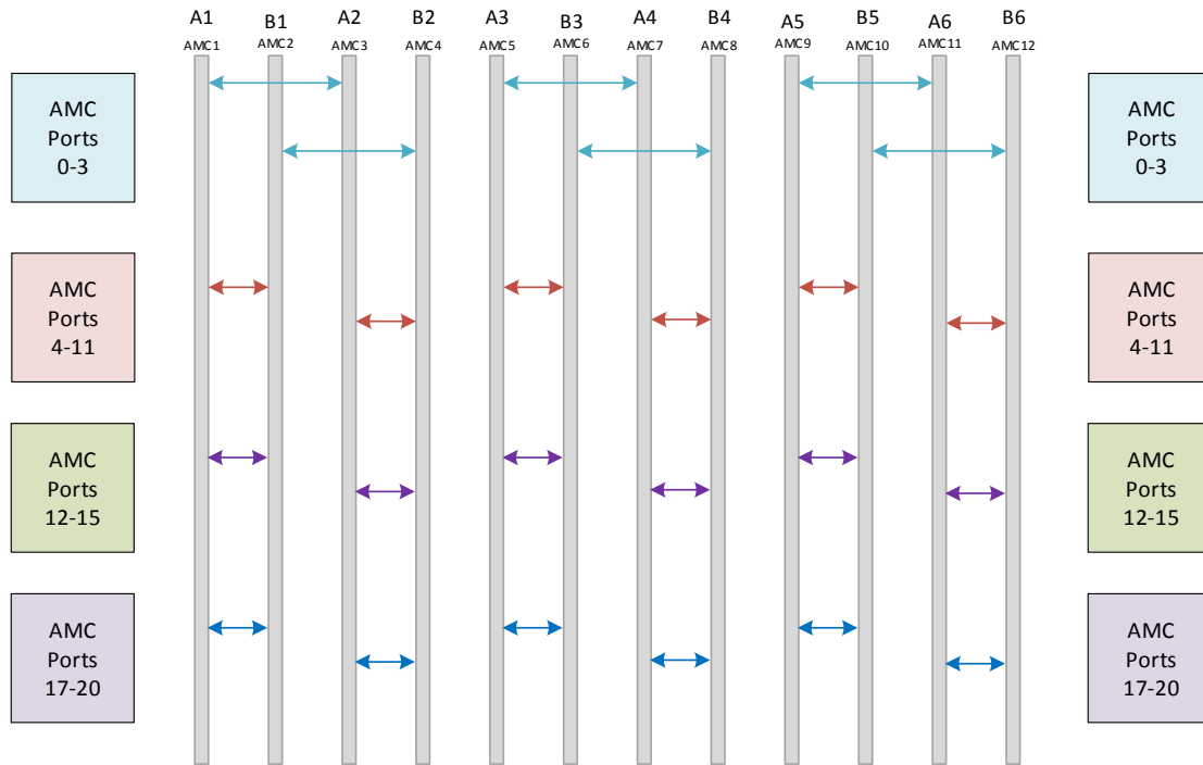
Figure 6: Backplane Connections on Secondary Connector (Tongue 2)
