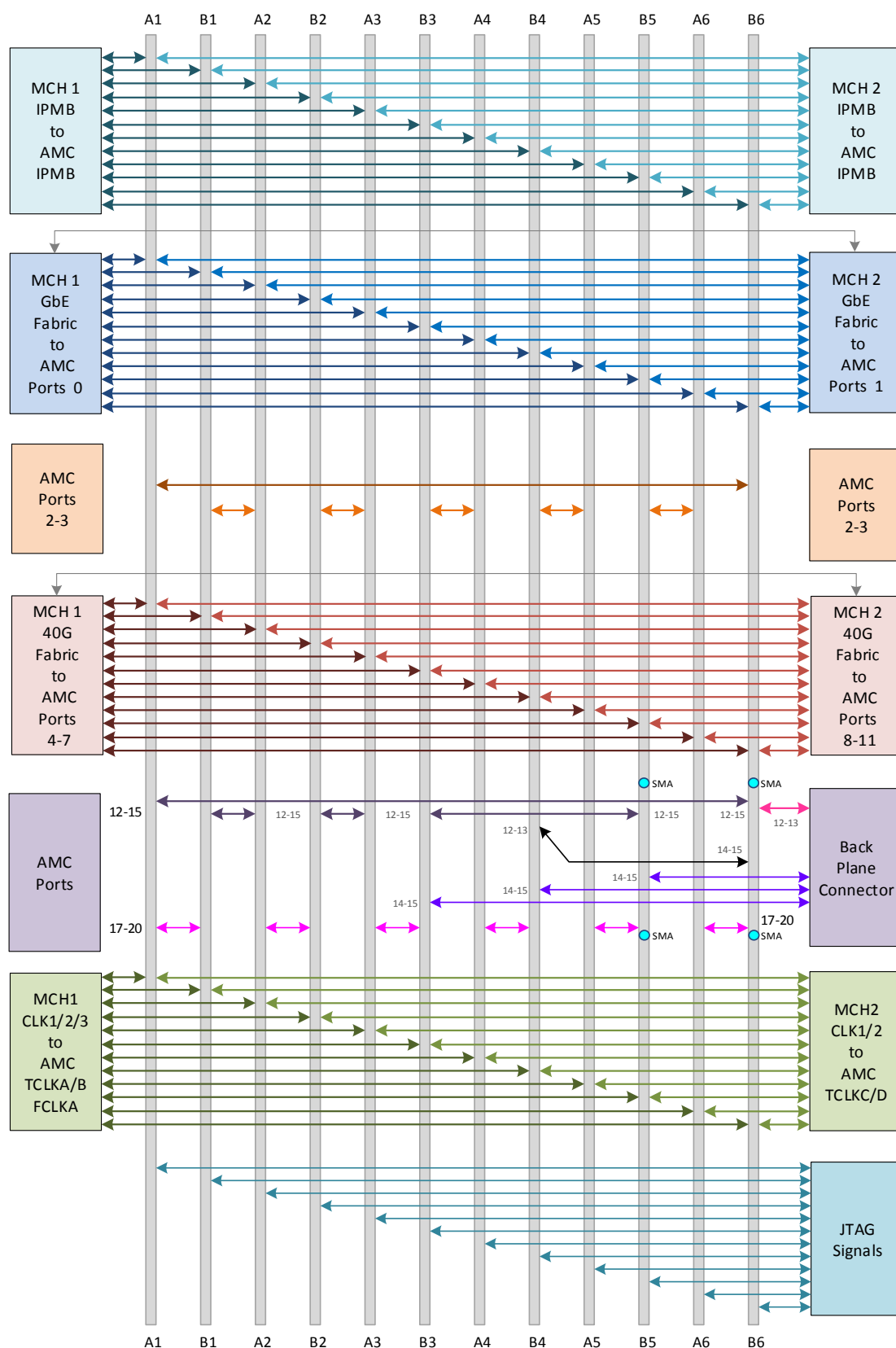
Figure 5: Backplane Connections on Primary AMC Connector
