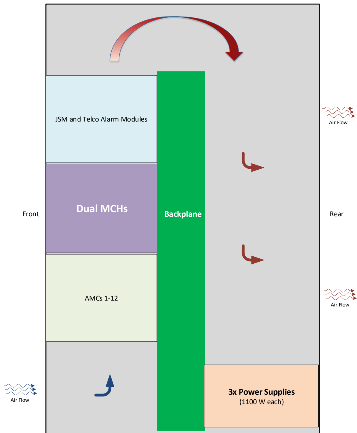
Figure 4: VT884 Top Level Functional Block Diagram
