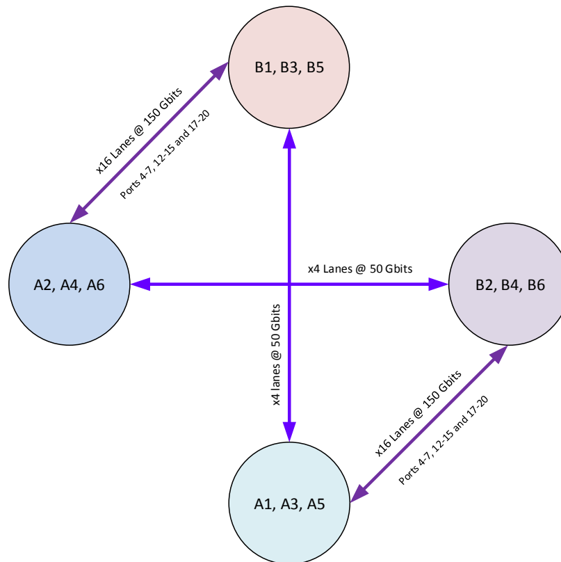
Figure 7: Backplane Speed on Secondary Connectors (Tongue 2)
