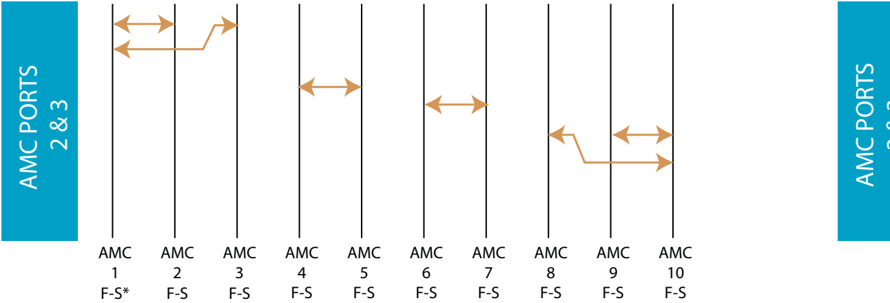
Topology for Ports 2 and 3 with direct connections among the slots (ordering option)
