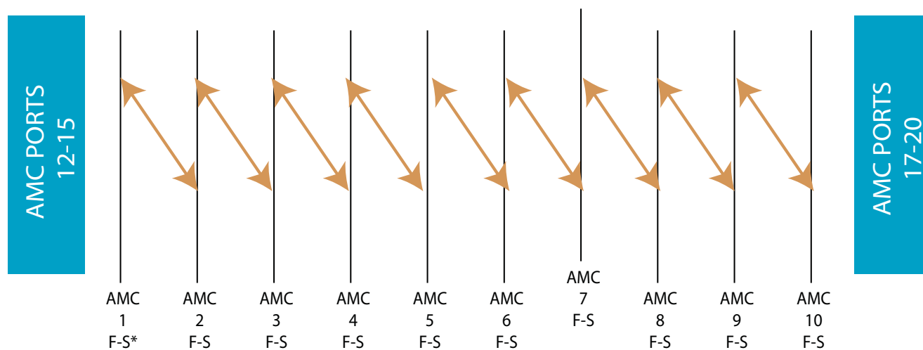
FIGURE 5. VT865 Topology for AMC Ports 12-15 and 17-20
