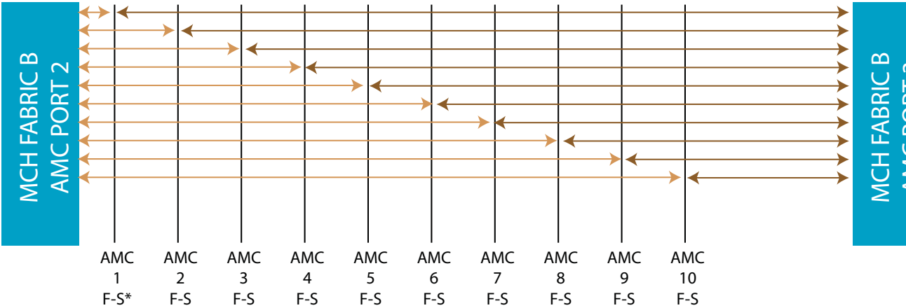
Topology for Ports 2 and 3 to MCH (ordering option with redundant CLK)
