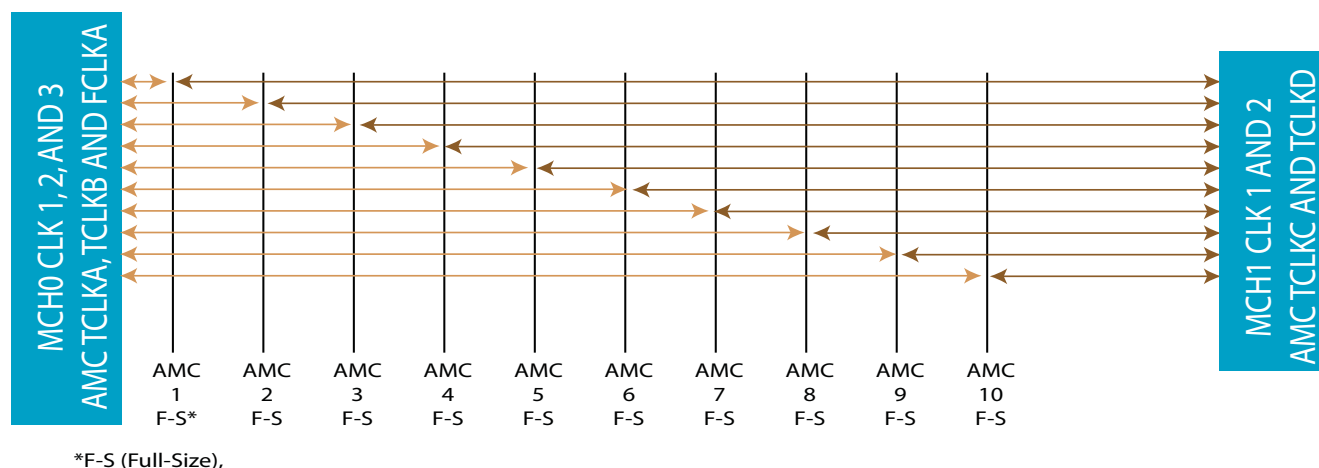
FIGURE 6. VT865 AMC 2.0 Enhanced Clock Redundancy Topology
