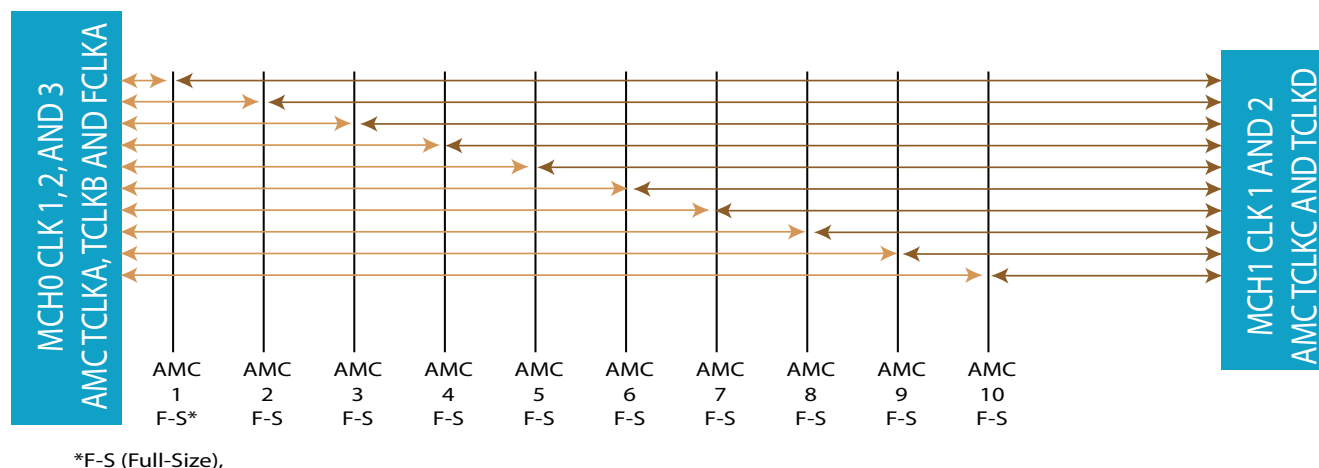
FIGURE 5. VT864 AMC 2.0 Enhanced Clock Redundancy Topology
