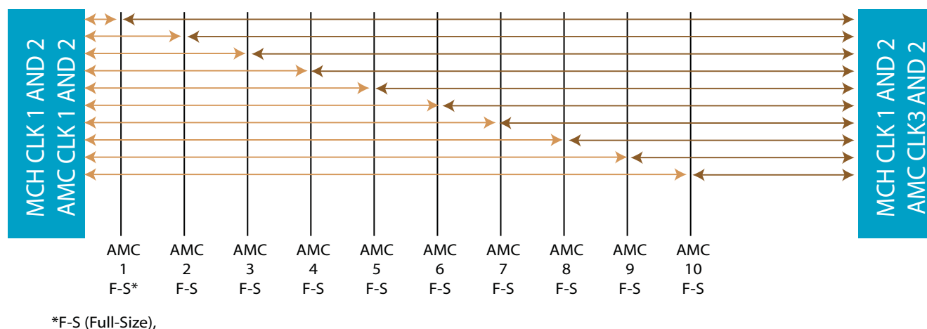
FIGURE 6. VT862 redundant clock Topology
