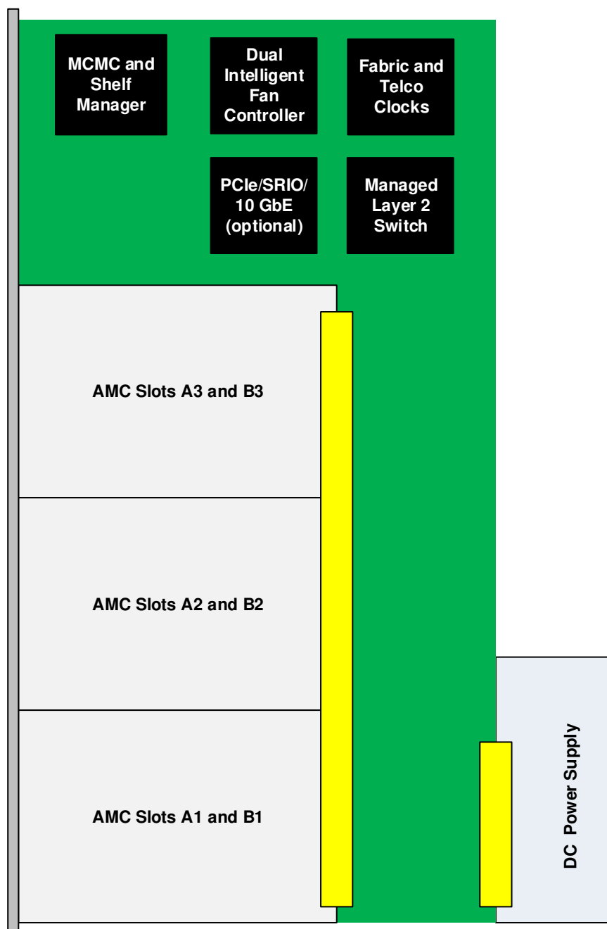
Figure 2: VT858 Block Diagram
