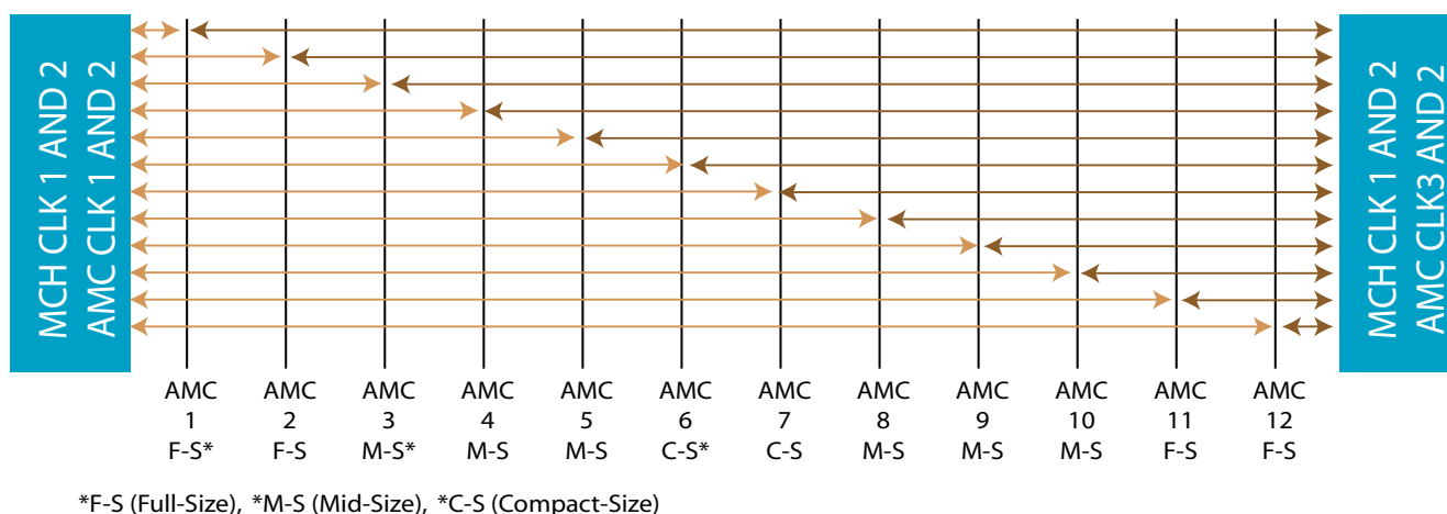
FIGURE 7. VT860 redundant clock Topology
