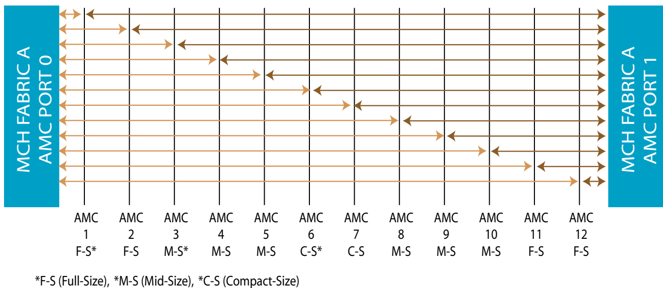
FIGURE 2. VT860 Topology for AMC Ports 0 and 1
