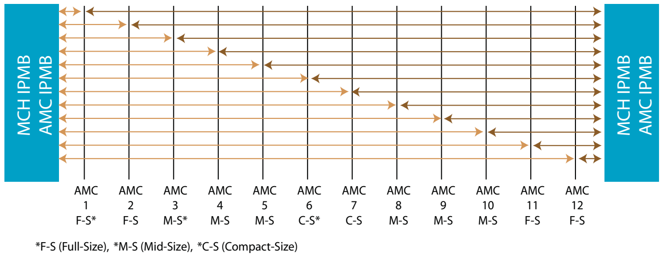
FIGURE 1. VT860 Topology for AMC I2C Bus
