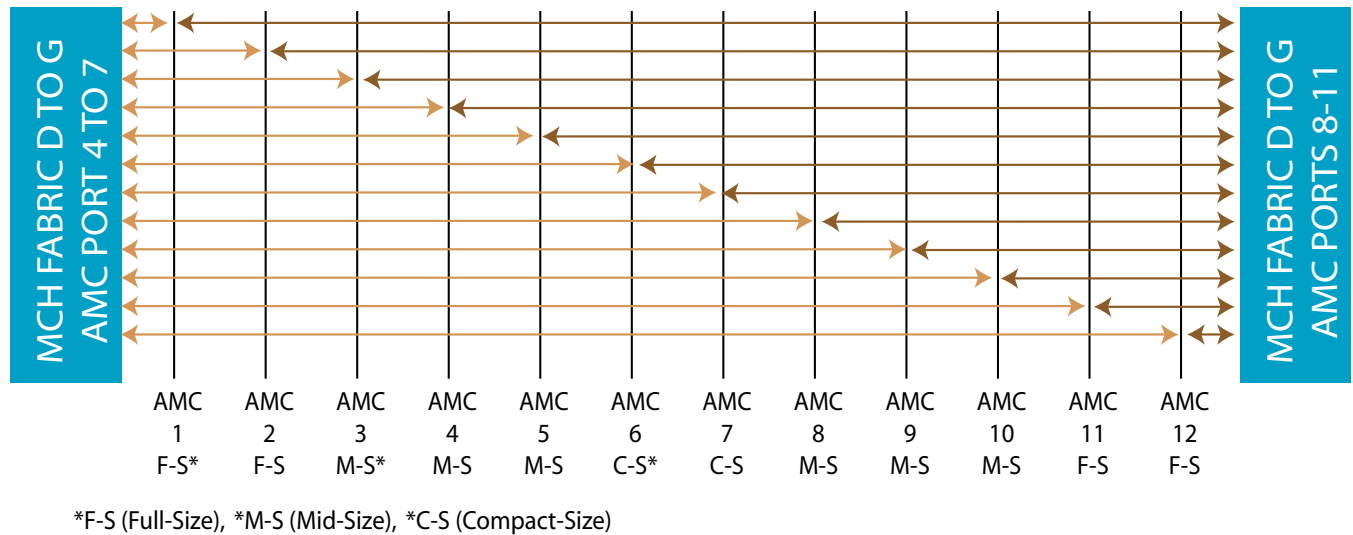
FIGURE 4. VT860 Topology for AMC Ports 4-7 and 8-11
