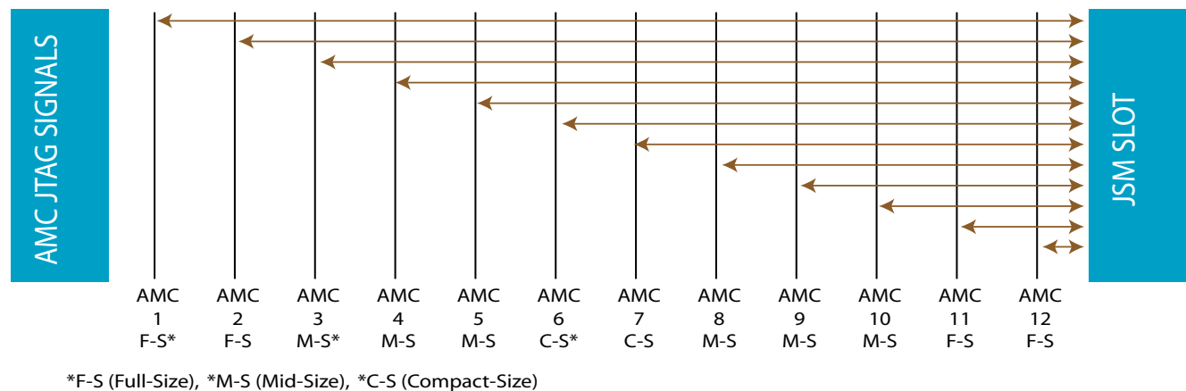
FIGURE 5. VT860 Topology for AMC JTAG Signals
