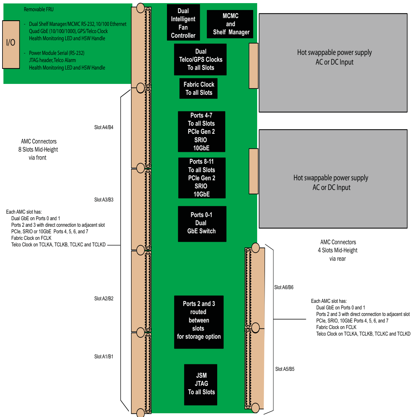
FIGURE 1. VT854 Functional Block Diagram
