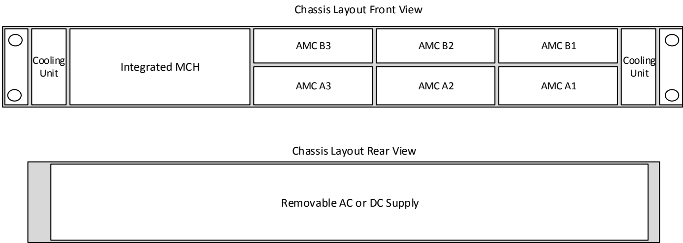
Figure 1: Chassis Layout
