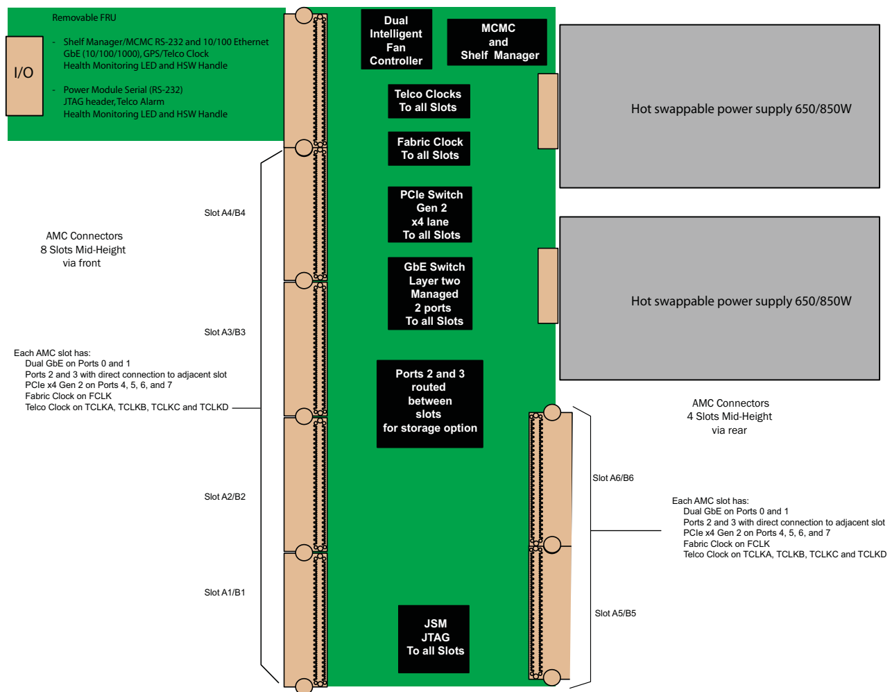
FIGURE 1. VT850 Functional Block Diagram
