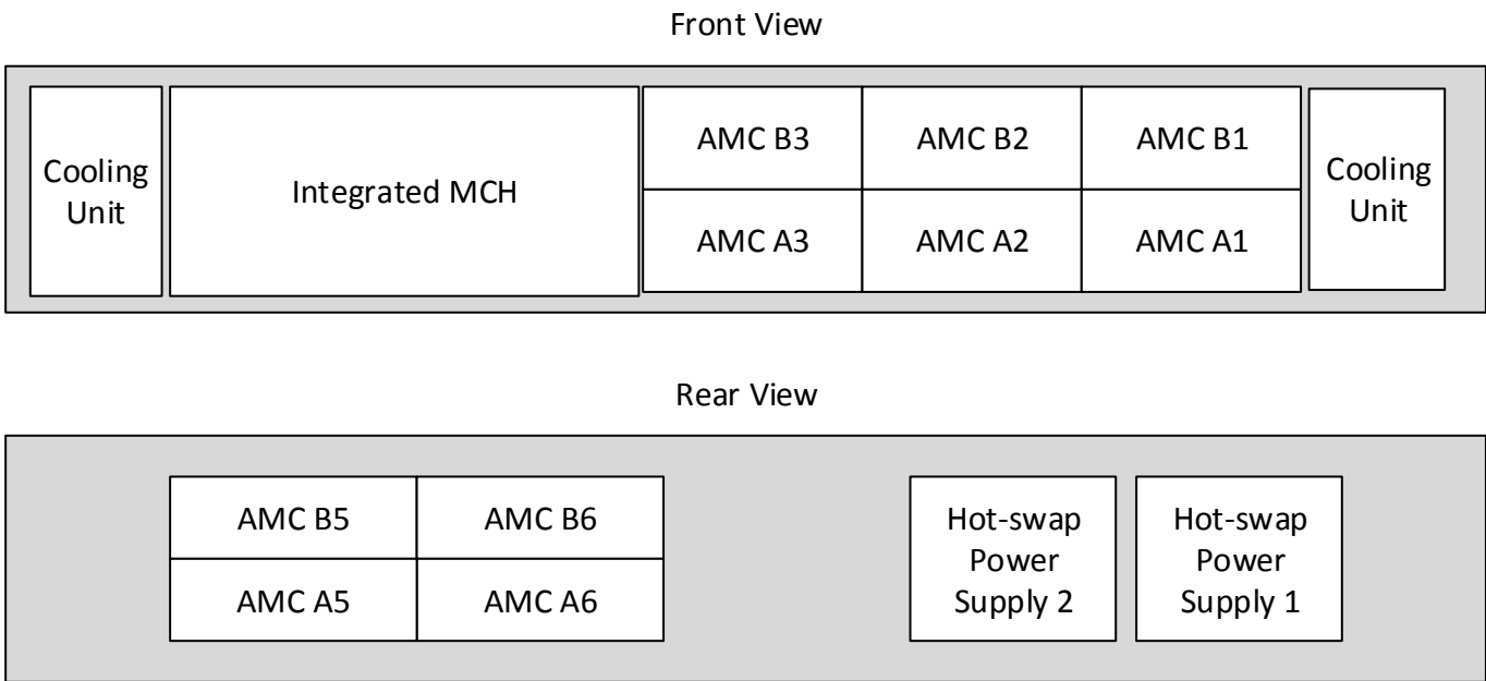
Figure 6: VT848 Chassis Layout
