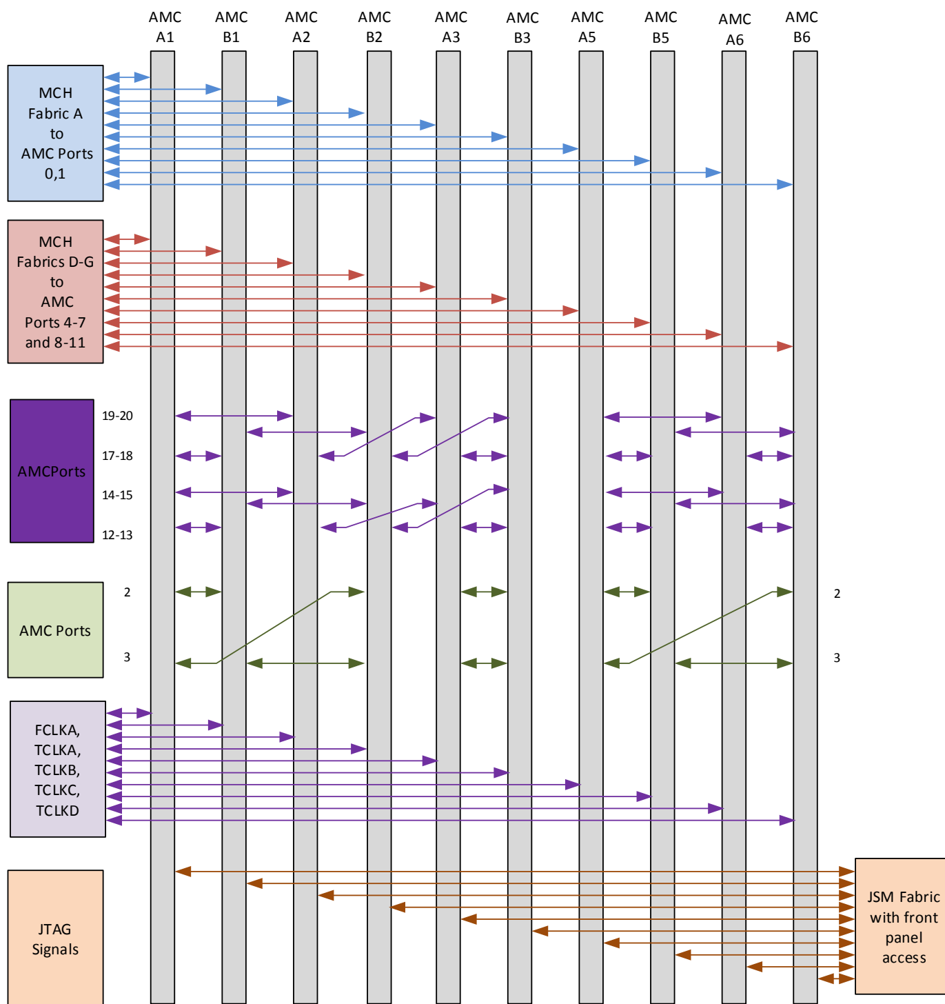
Figure 5: VT848 Backplane Connections
