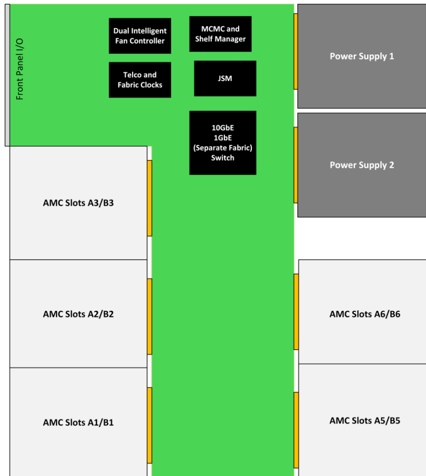
Figure 3: VT848 Block Diagram
