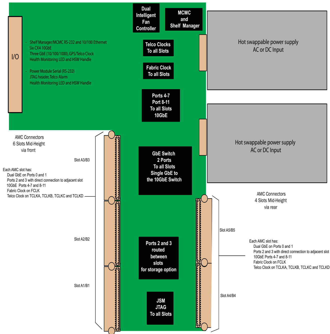
FIGURE 1. VT847 Functional Block Diagram
