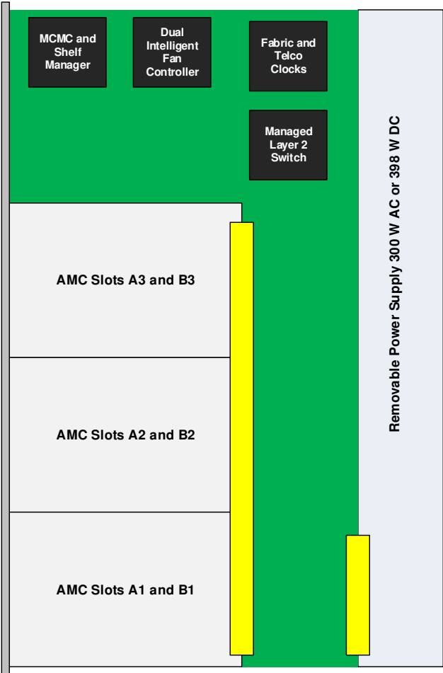
Figure 4: VT842 Functional Block Diagram
