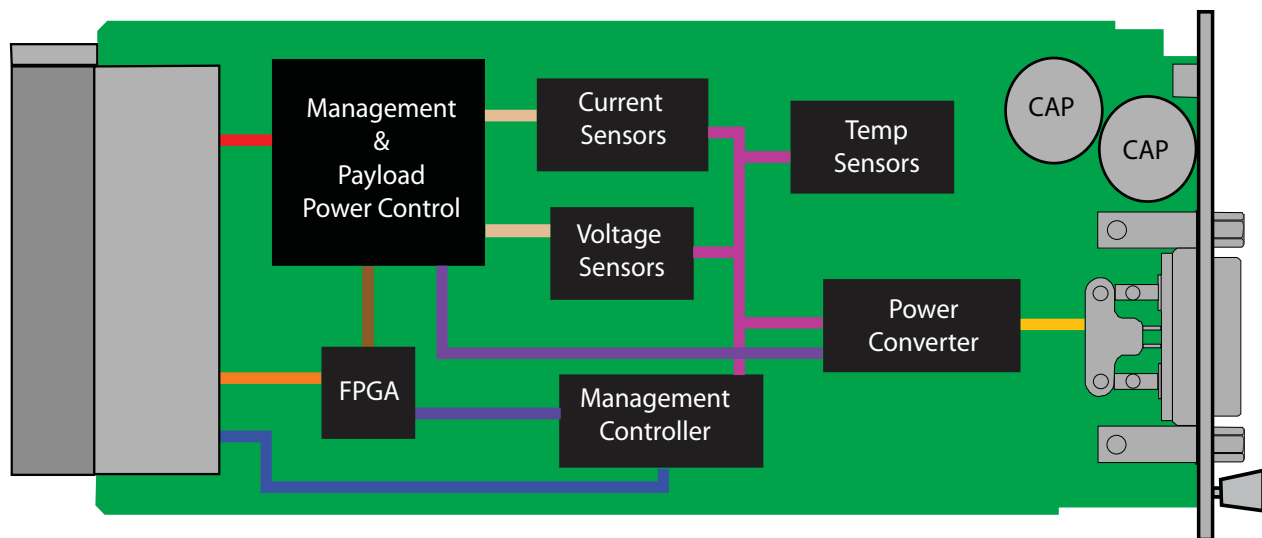
FIGURE 1. UTC011 Functional Block Diagram
