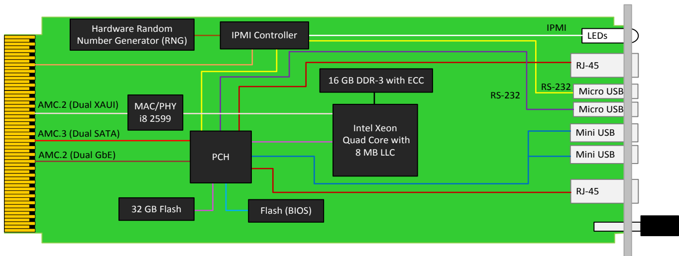
Figure 1: AMC721 Functional Block Diagram
