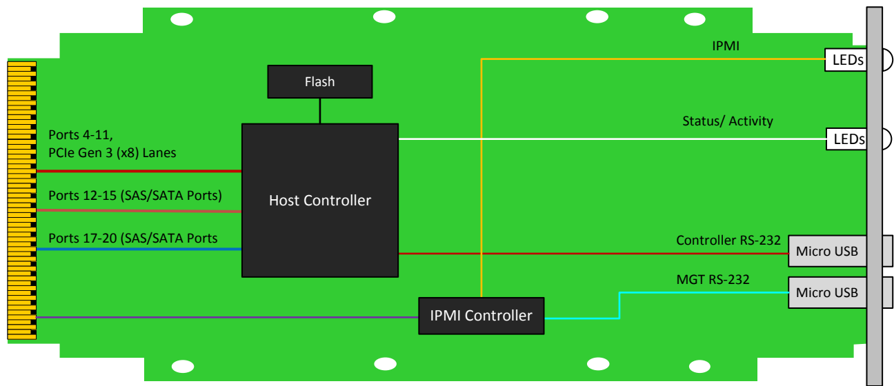
Figure 3: AMC629C Block Diagram
