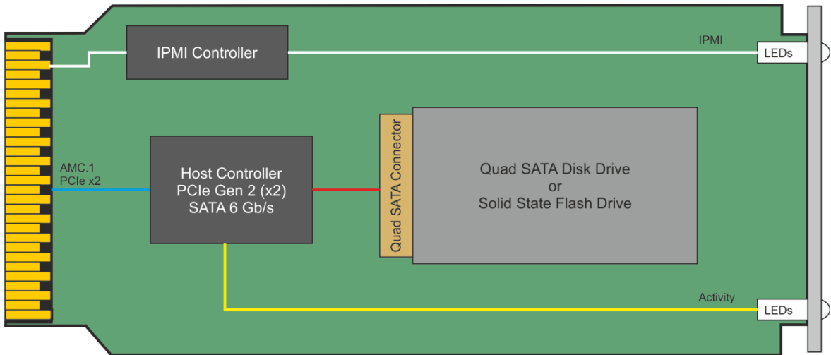
Figure 1: Block Diagram
