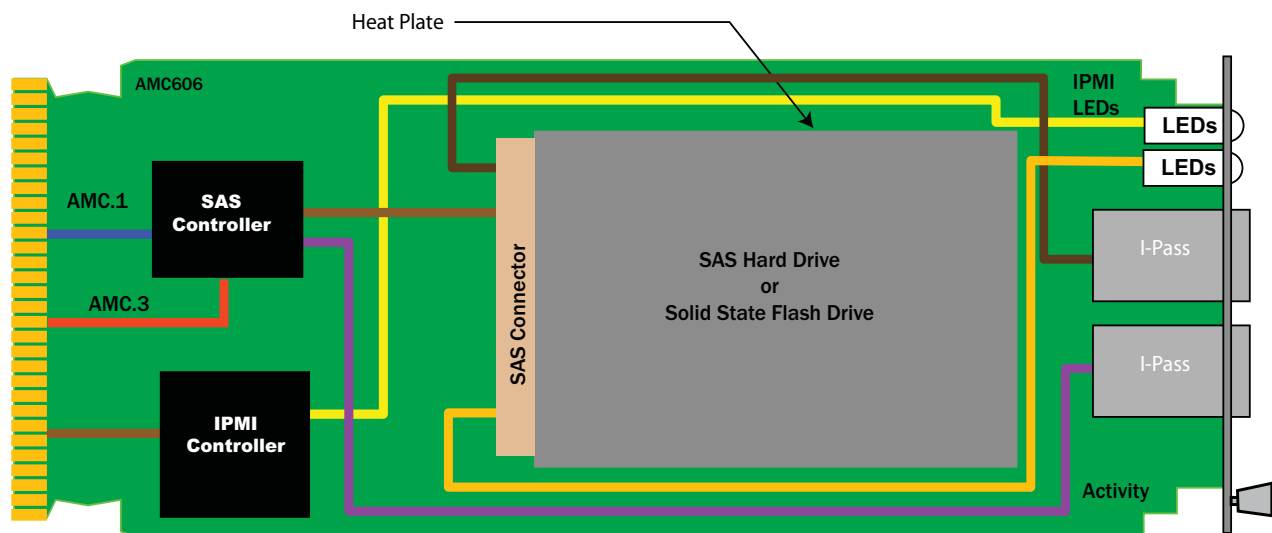
FIGURE 1. AMC606 Functional Block Diagram
