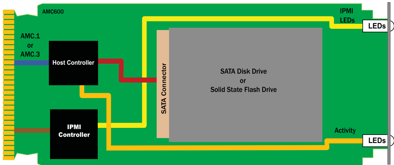
FIGURE 1. AMC600 Functional Block Diagram
