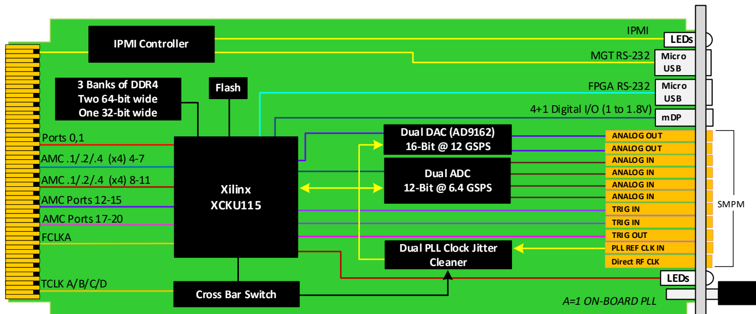
Figure 3: Functional Block Diagram for Option A = 1
