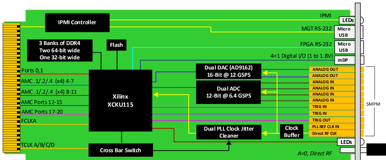
Figure 2: Functional Block Diagram for Option A = 0
