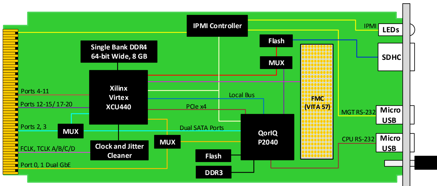
Figure 2: AMC595 Functional Block Diagram
