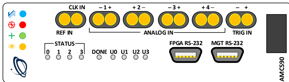
Figure 3: AMC590 Front Panel
