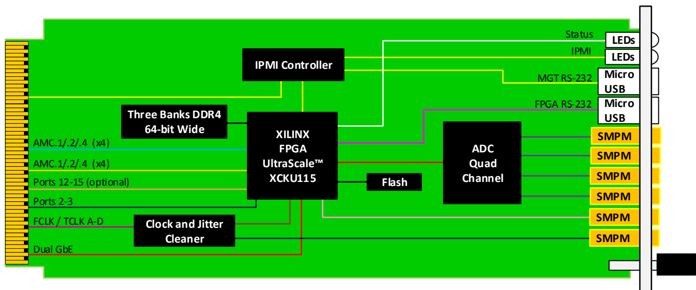
Figure 2: AMC590 Functional Block Diagram
