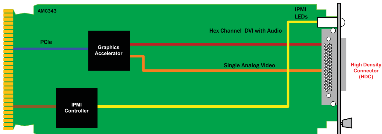
FIGURE 1. AMC343 Functional Block Diagram
