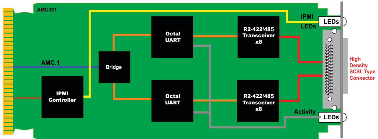
FIGURE 1. AMC321 Functional Block Diagram
