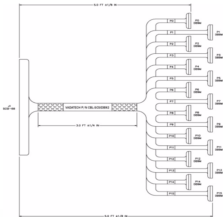
FIGURE 3. Adapter Cable
