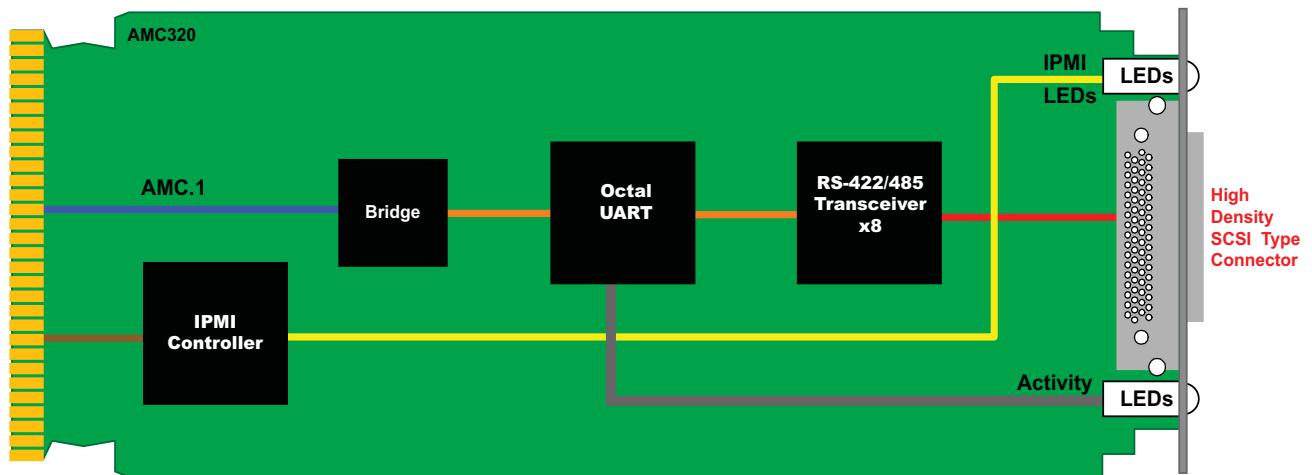
FIGURE 1. AMC320 Functional Block Diagram
