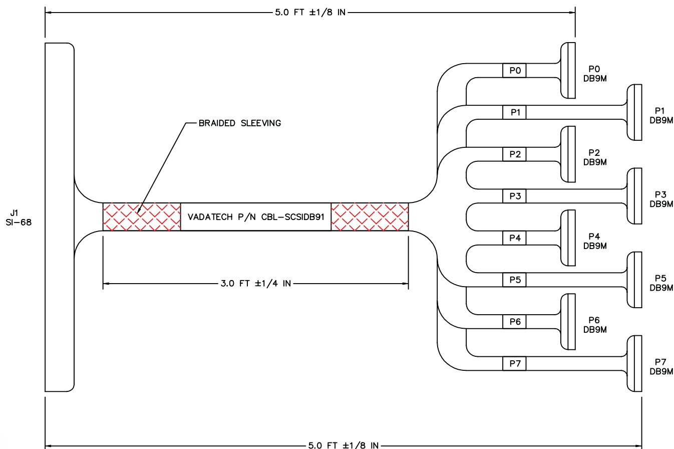
FIGURE 3. Front Panel Adapter Cable
