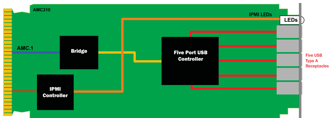
FIGURE 1. AMC310 Functional Block Diagram
