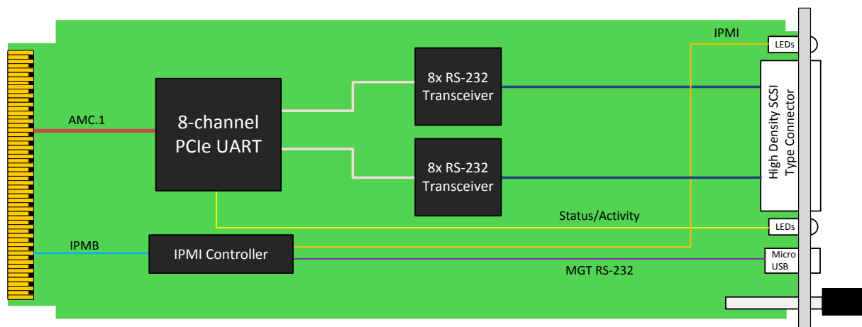
Figure 1: AMC304 Block Diagram and Front Panel
