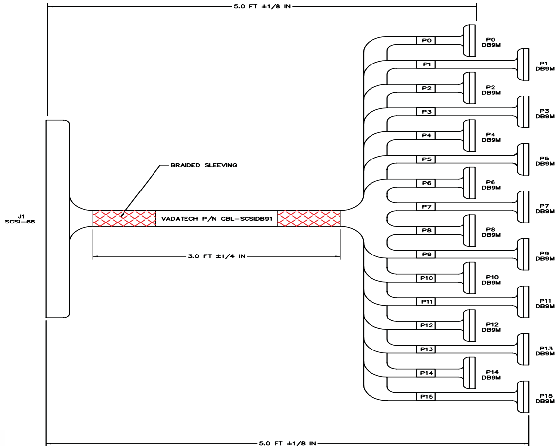
FIGURE 3. Front Panel Adapter Cable
