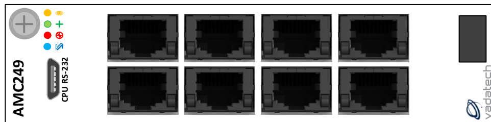
Figure 3: AMC249 Front Panel View
