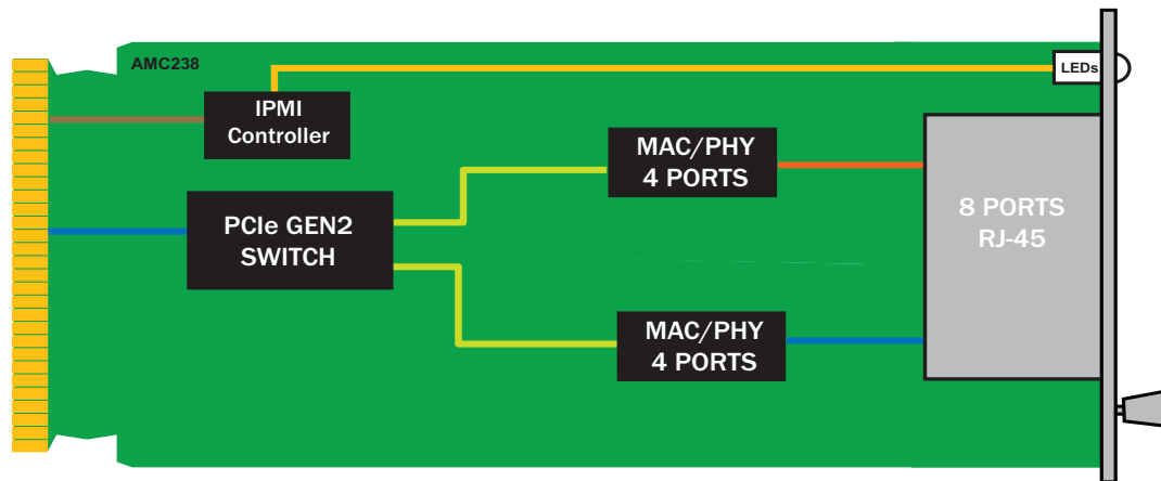
FIGURE 1. AMC238 Functional Block Diagram
