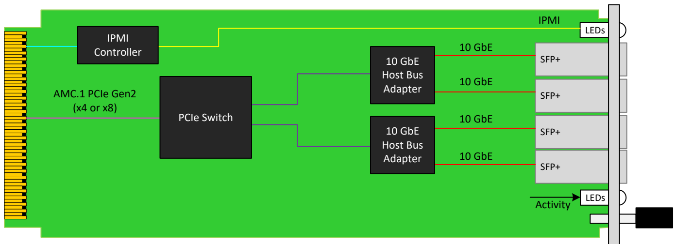
Figure 2: AMC231 Functional Block Diagram
