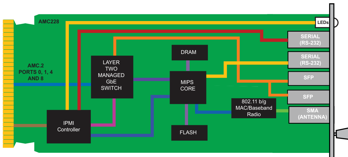
FIGURE 1. AMC228 Functional Block Diagram
