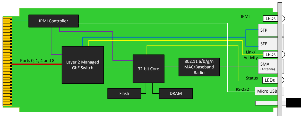
Figure 1: AMC227 Block Diagram
