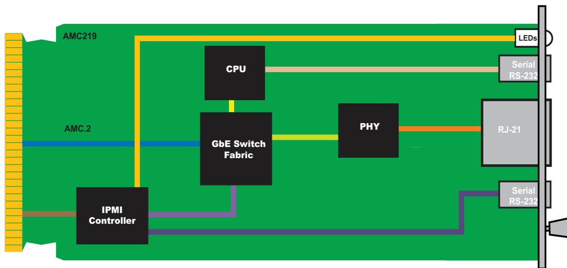
FIGURE 1. AMC219 Functional Block Diagram
