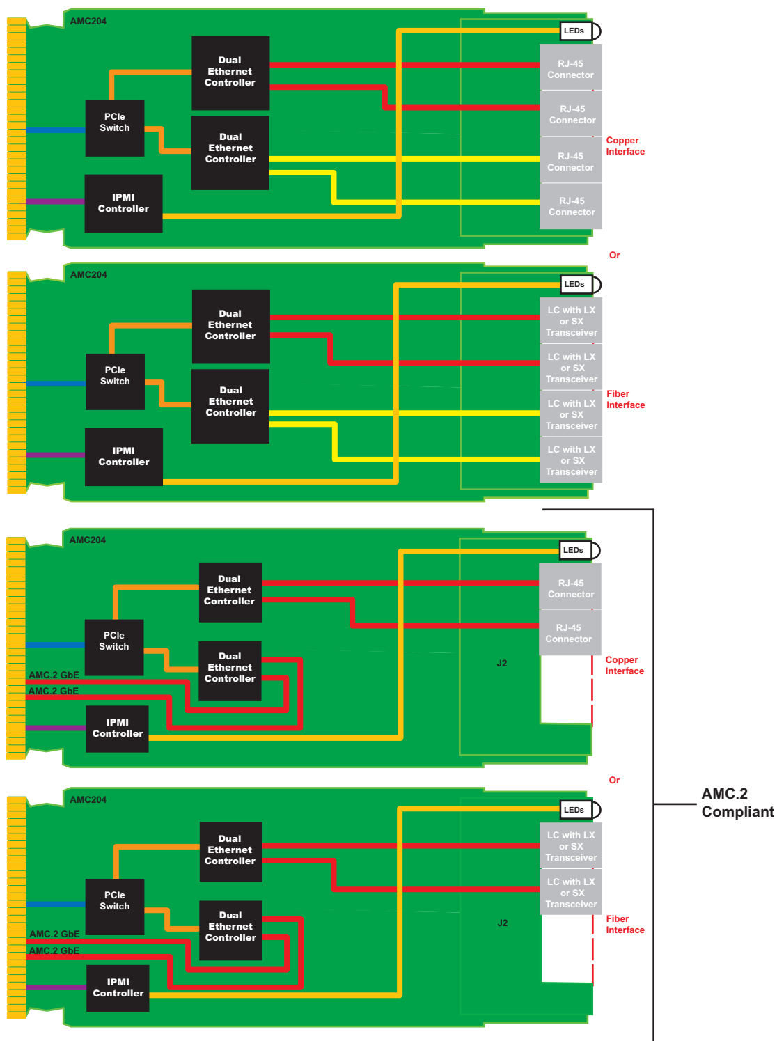
FIGURE 1. AMC204 Functional Block Diagram
