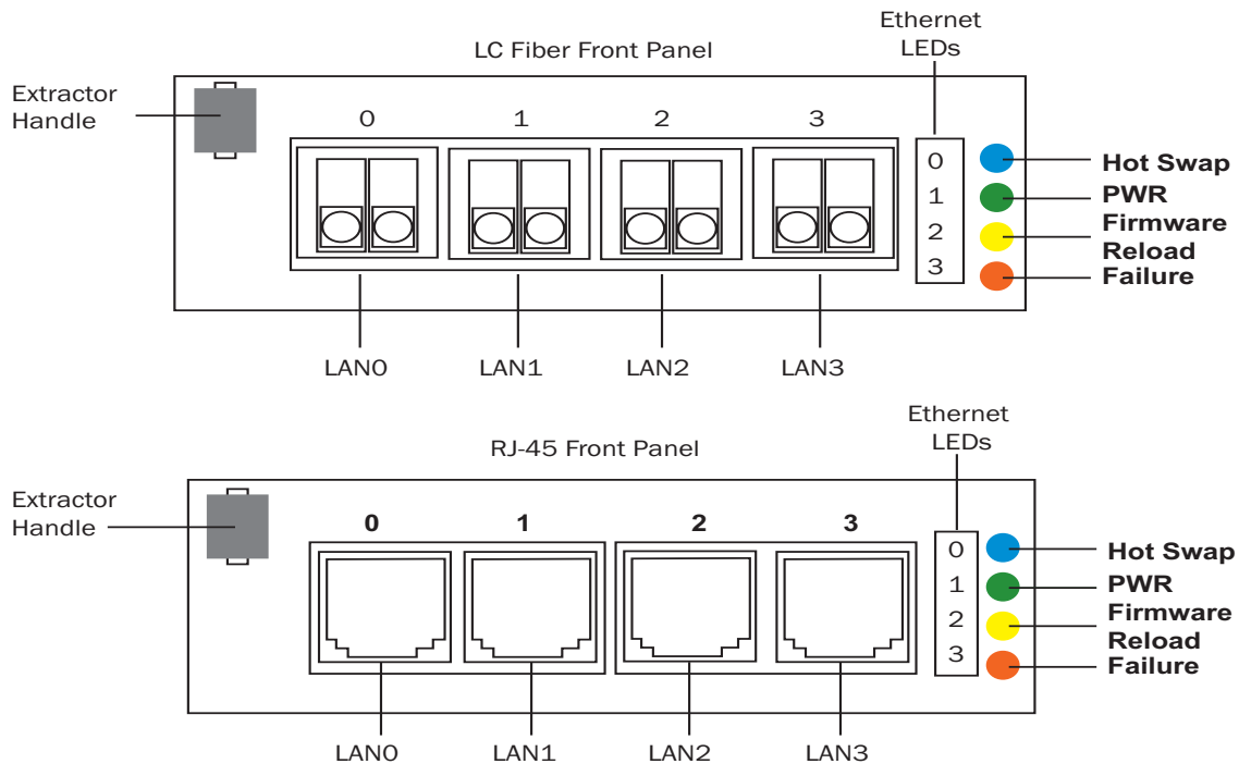
FIGURE 2. AMC204 Front Panels
