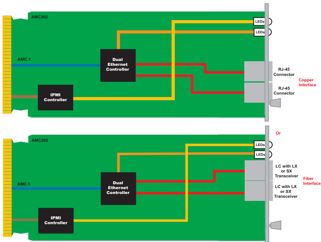
FIGURE 1. AMC202 Functional Block Diagram
