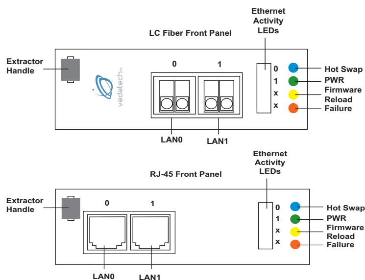
FIGURE 2. AMC202 Front Panels
