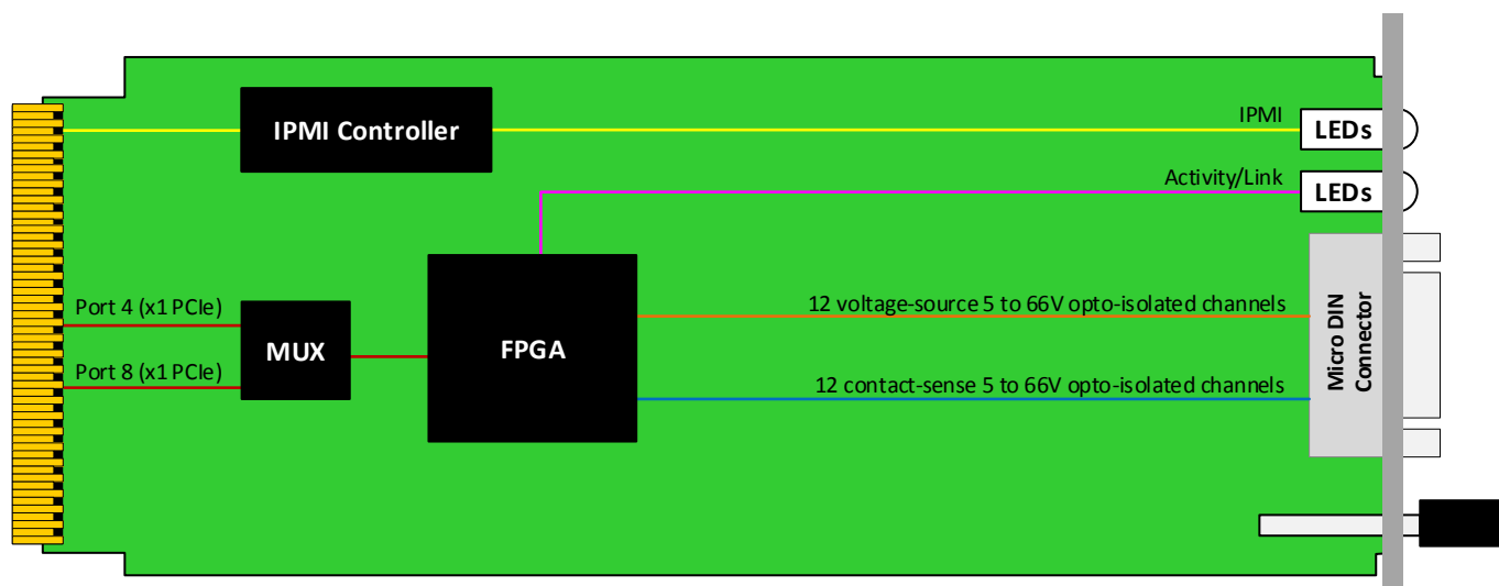
Figure 1: Block Diagram
