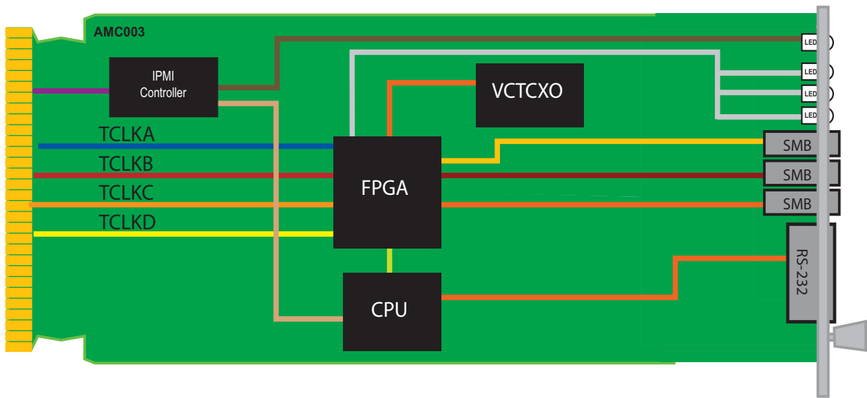
FIGURE 1. AMC003 Functional Block Diagram
